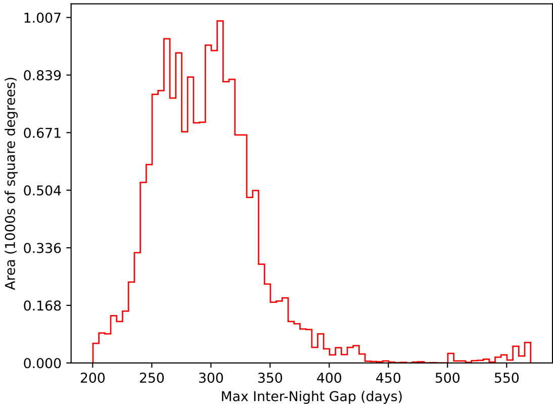
weather_cloudso14v3.4_10yrs WFD i band: Max Inter-Night Gap
