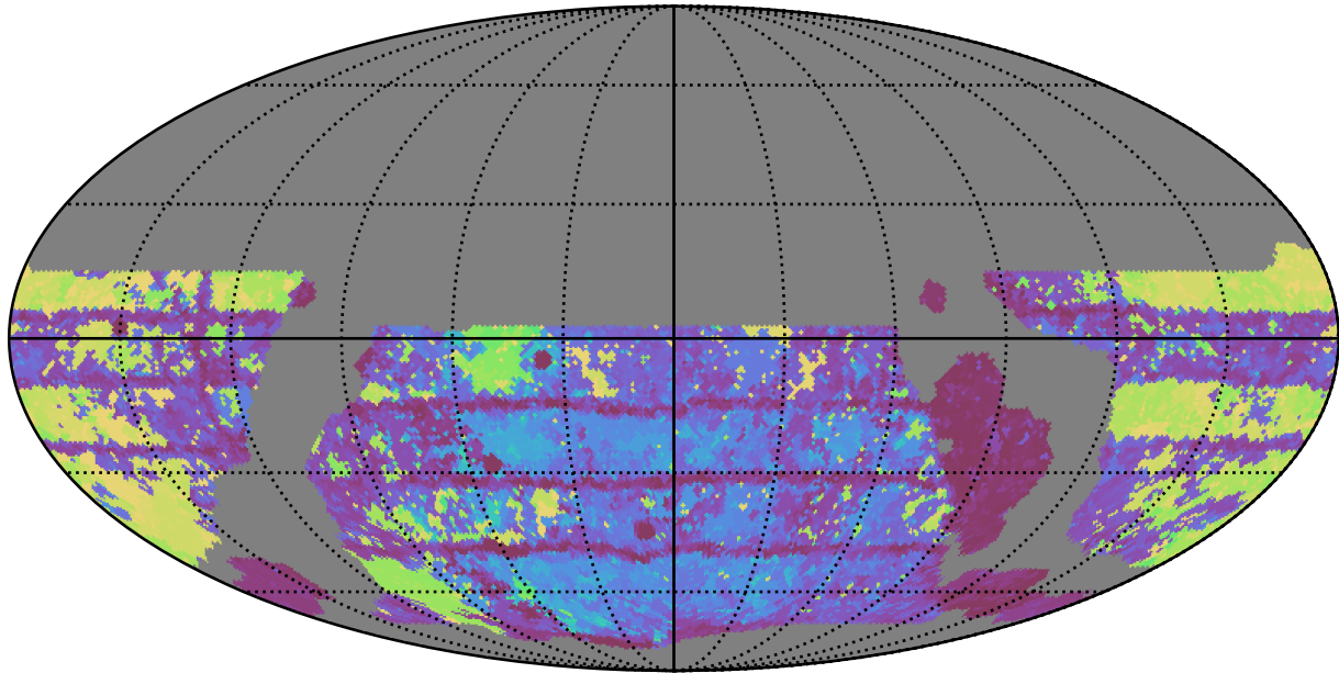
weather_cloudso14v3.4_10yrs WFD g band: Max Inter-Night Gap
