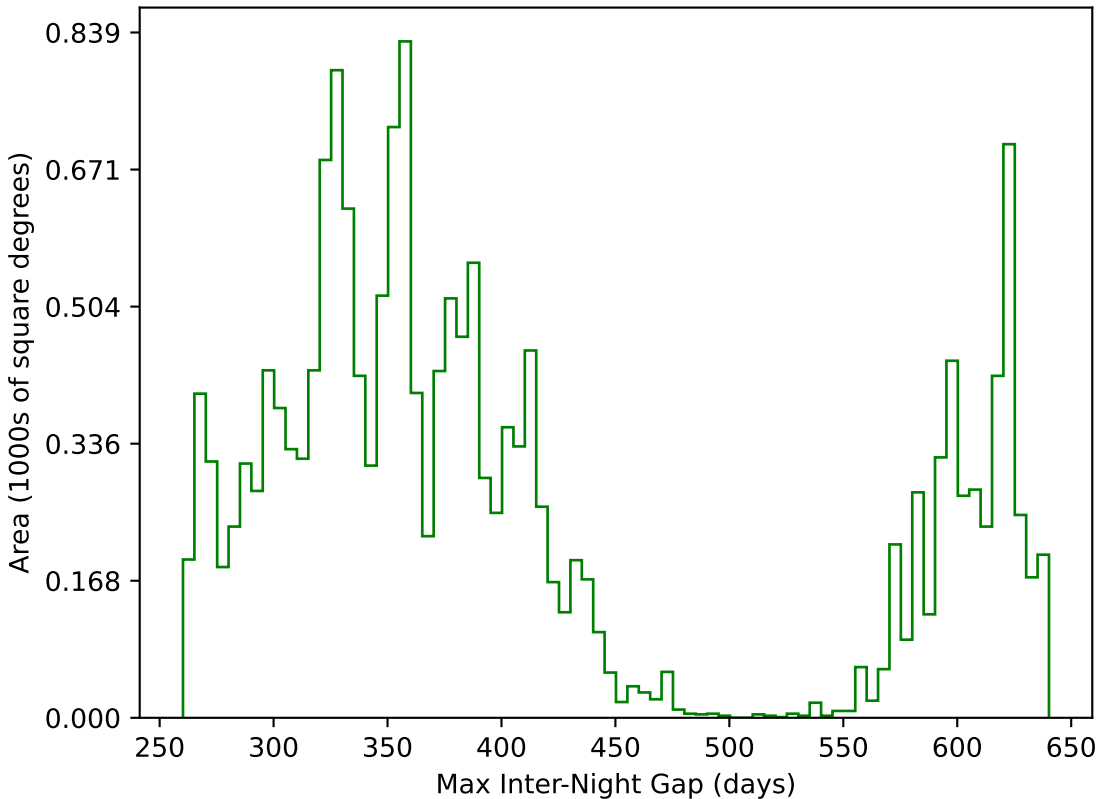
weather_cloudso14v3.4_10yrs WFD g band: Max Inter-Night Gap
