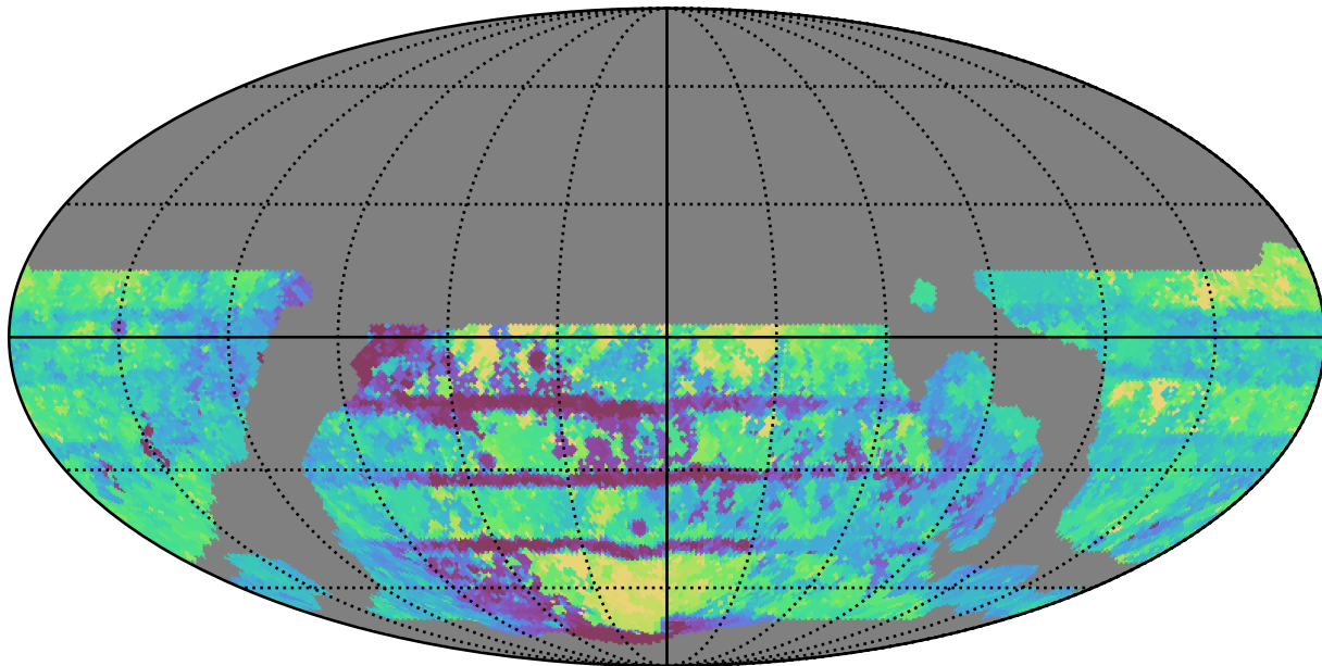
weather_cloudso14v3.4_10yrs WFD all bands: Max Inter-Night Gap
