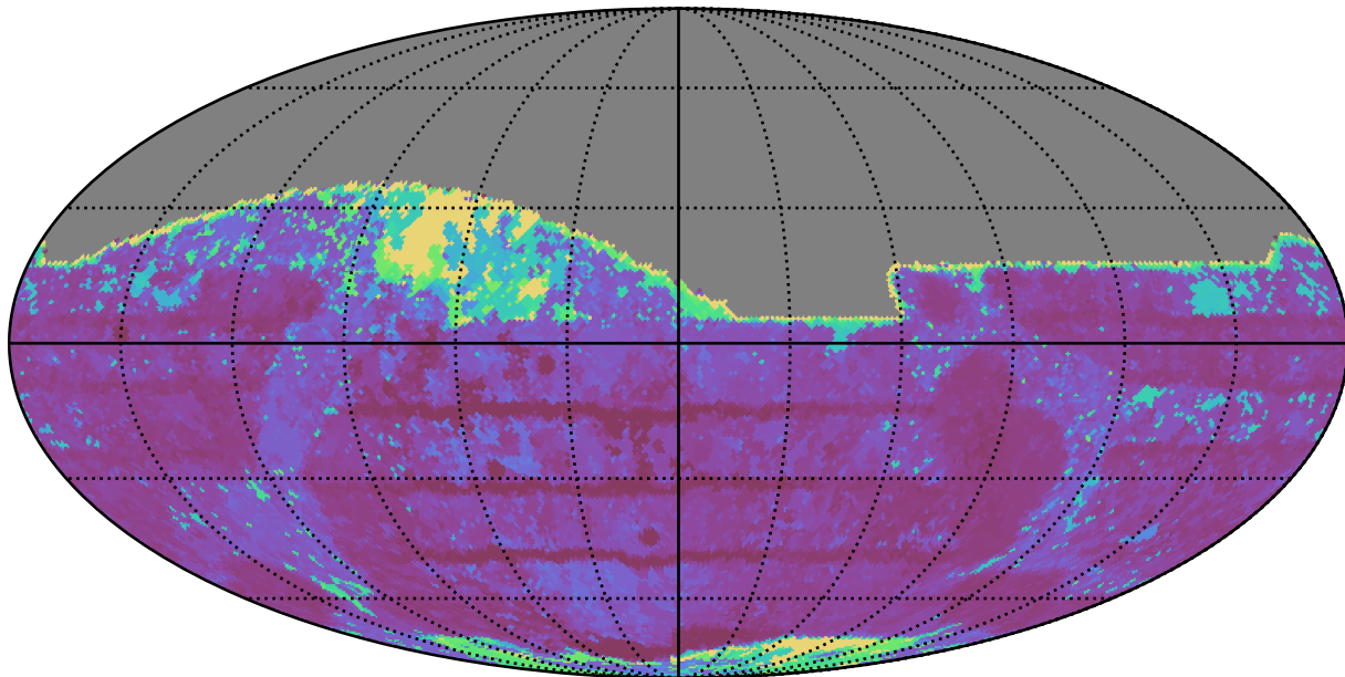
weather_cloudso14v3.4_10yrs All sky z band: Max Inter-Night Gap
