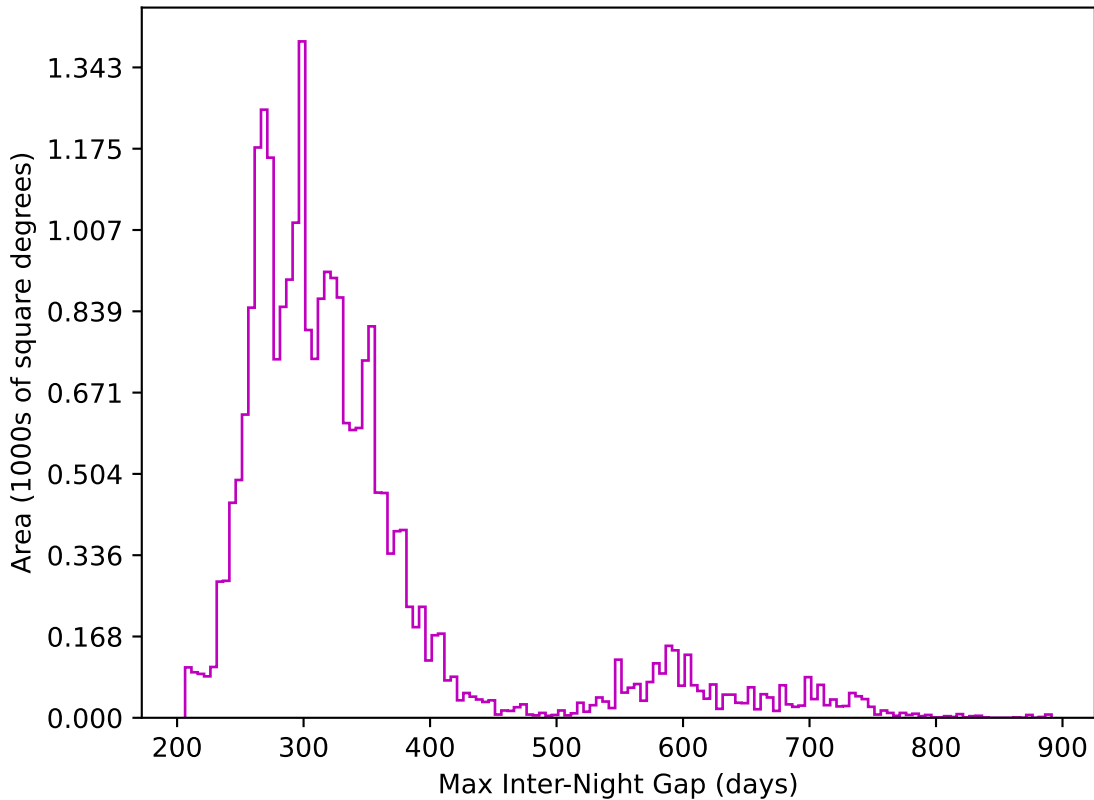
weather_cloudso14v3.4_10yrs All sky z band: Max Inter-Night Gap
