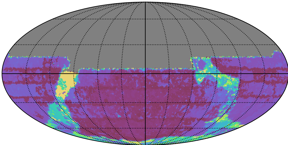
weather_cloudso14v3.4_10yrs All sky u band: Max Inter-Night Gap
