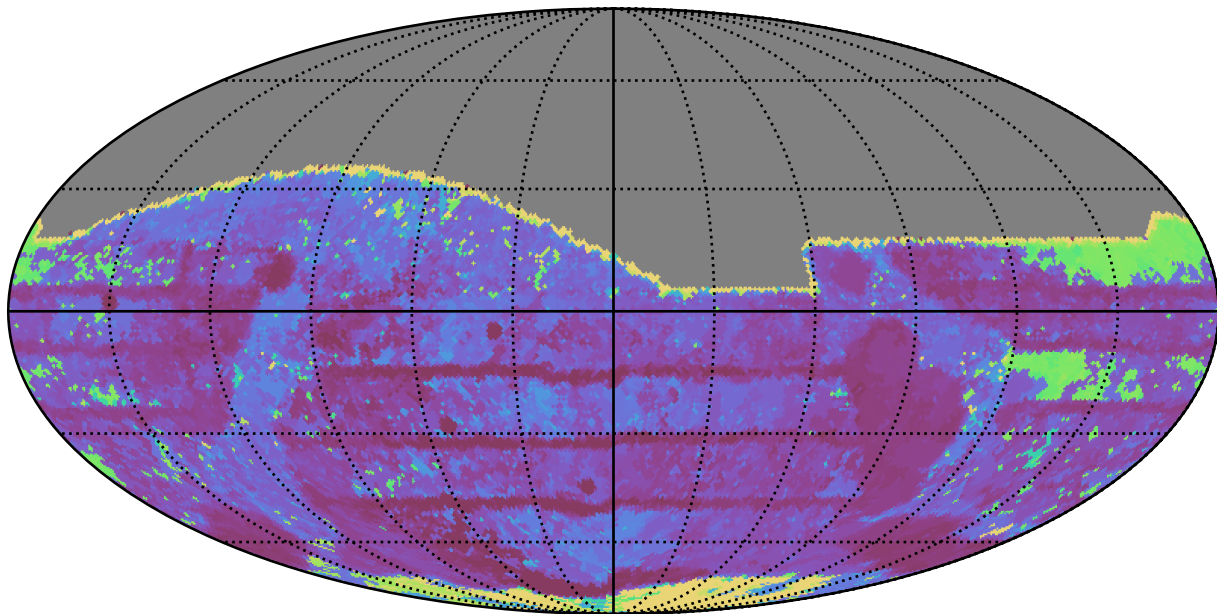
weather_cloudso14v3.4_10yrs All sky r band: Max Inter-Night Gap
