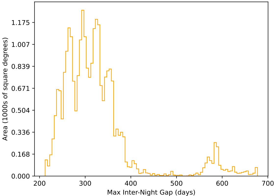
weather_cloudso14v3.4_10yrs All sky r band: Max Inter-Night Gap
