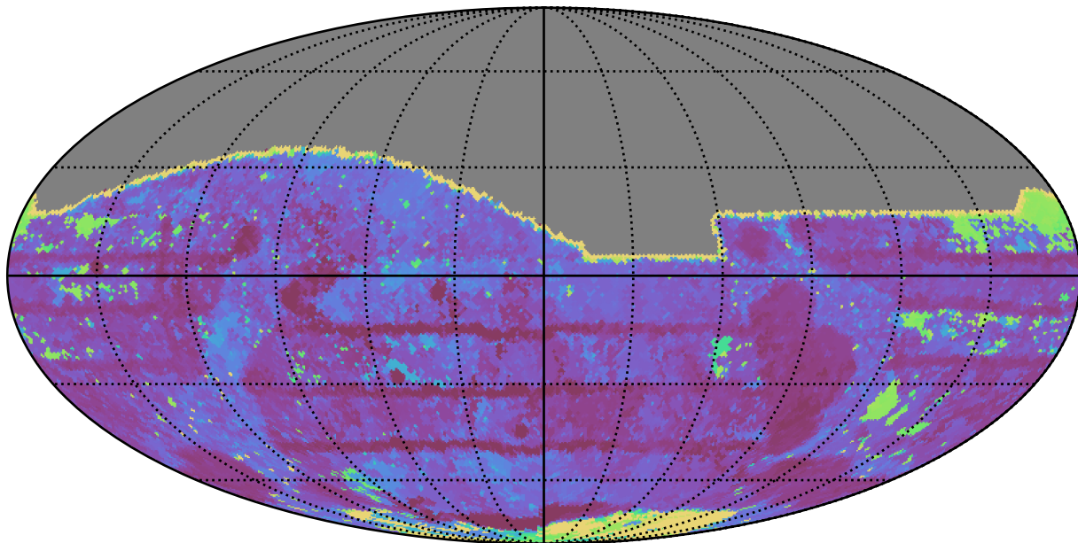
weather_cloudso14v3.4_10yrs All sky i band: Max Inter-Night Gap
