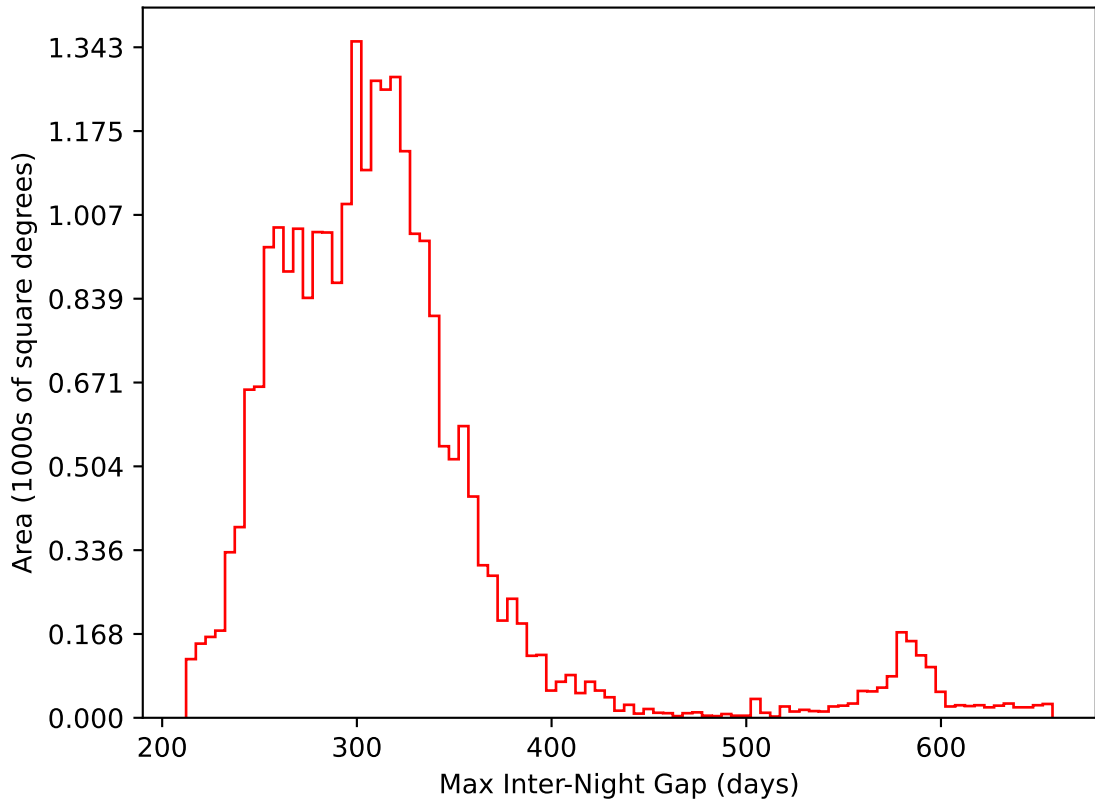
weather_cloudso14v3.4_10yrs All sky i band: Max Inter-Night Gap
