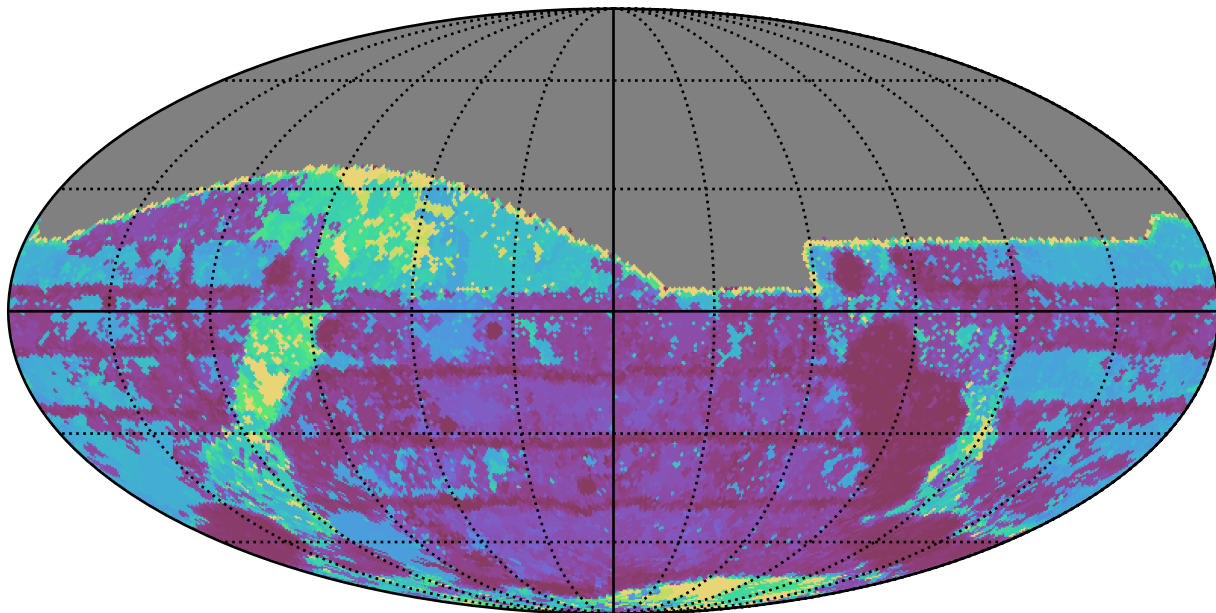
weather_cloudso14v3.4_10yrs All sky g band: Max Inter-Night Gap
