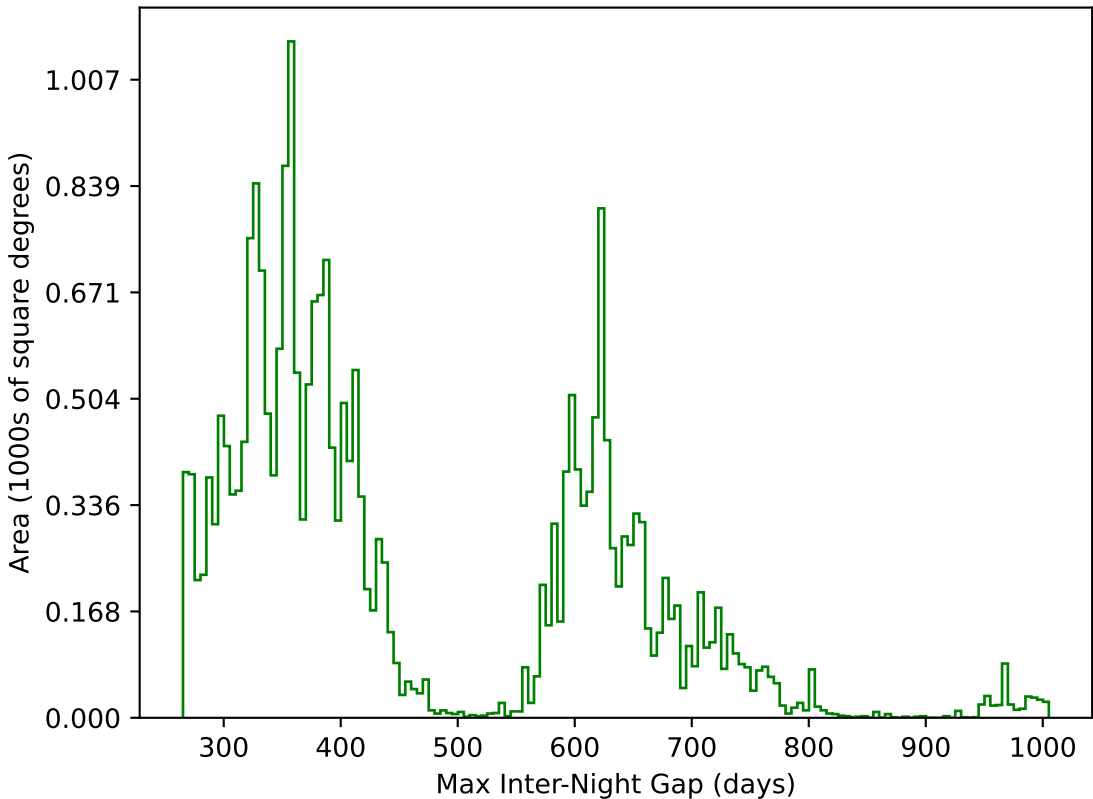
weather_cloudso14v3.4_10yrs All sky g band: Max Inter-Night Gap
