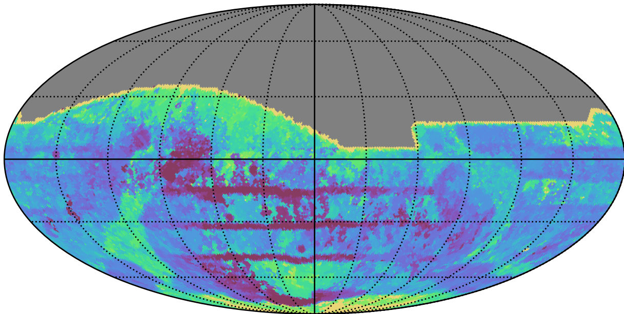
weather_cloudso14v3.4_10yrs All sky all bands: Max Inter-Night Gap
