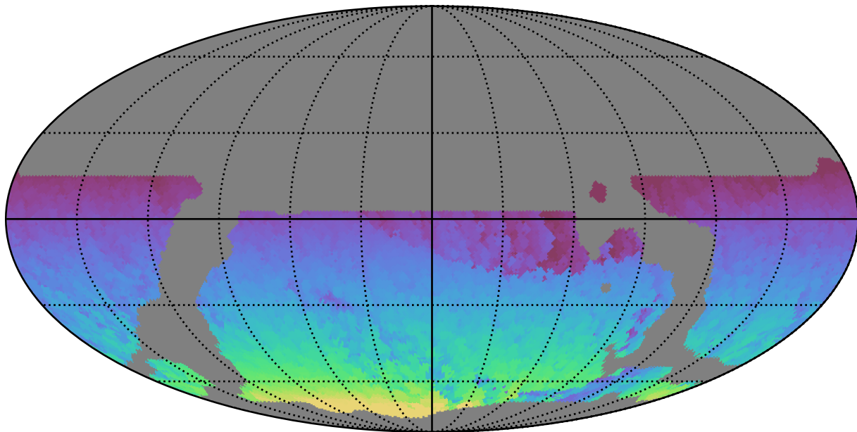
weather_cloudso14v3.4_10yrs WFD all bands: Max HA
