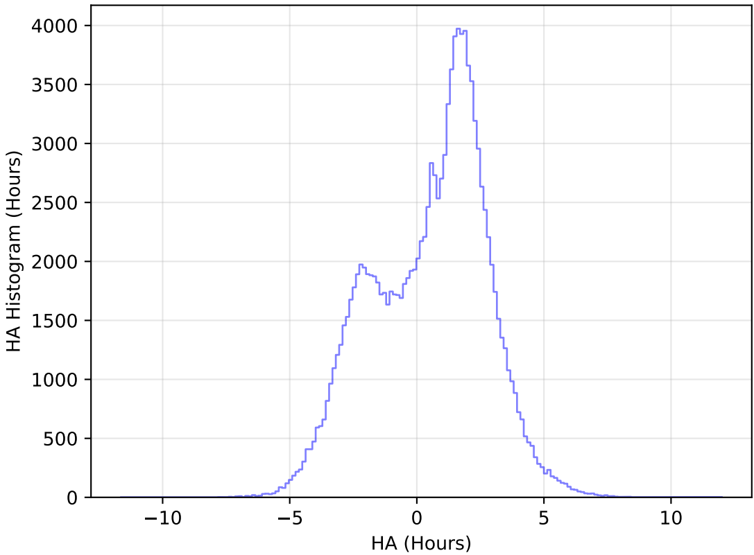
weather_cloudso14v3.4_10yrs WFD u band: HA Histogram
