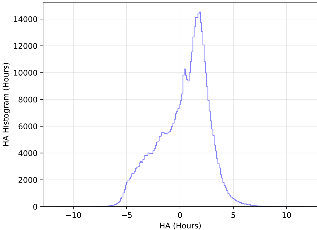
weather_cloudso14v3.4_10yrs WFD r band: HA Histogram
