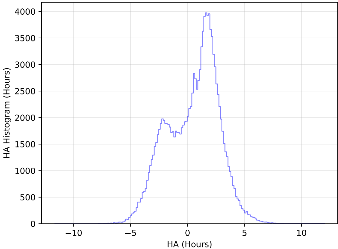
weather_cloudso14v3.4_10yrs All sky u band: HA Histogram
