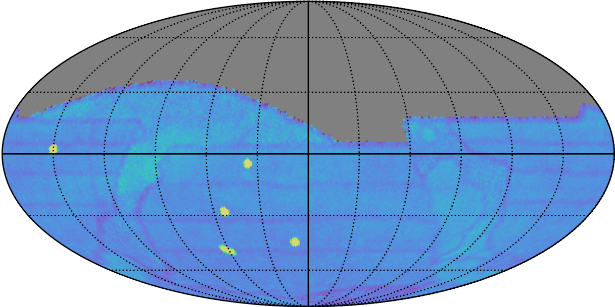
weather_cloudso14v3.4_10yrs gri All sky: Fraction of visits with a revisit < 60 min
