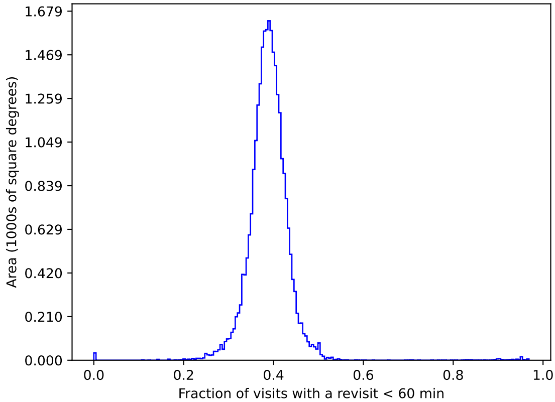
weather_cloudso14v3.4_10yrs gri All sky: Fraction of visits with a revisit < 60 min
