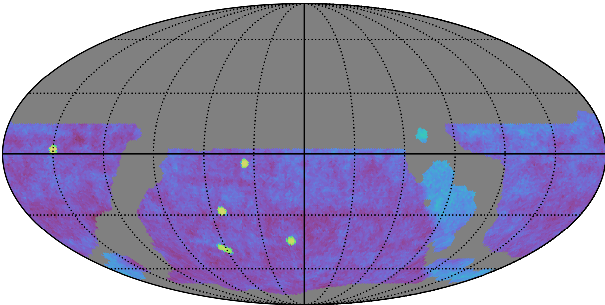
weather_cloudso14v3.4_10yrs gri WFD: Fraction of visits in pairs (10-60 min)
