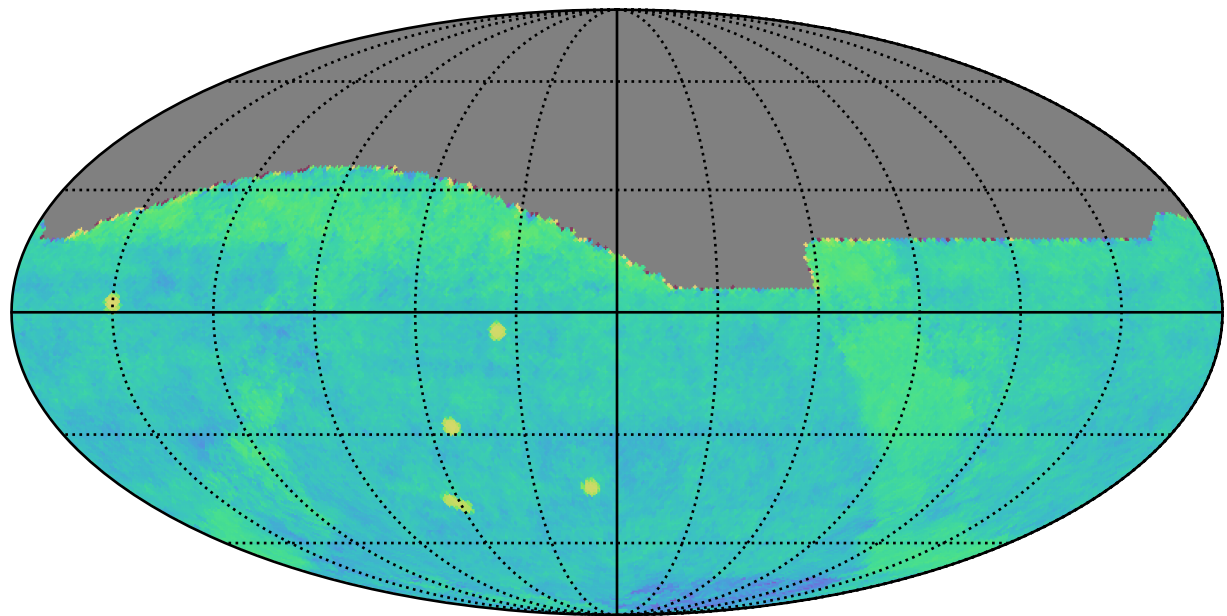
weather_cloudso14v3.4_10yrs gri All sky: Fraction of visits in pairs (10-60 min)
