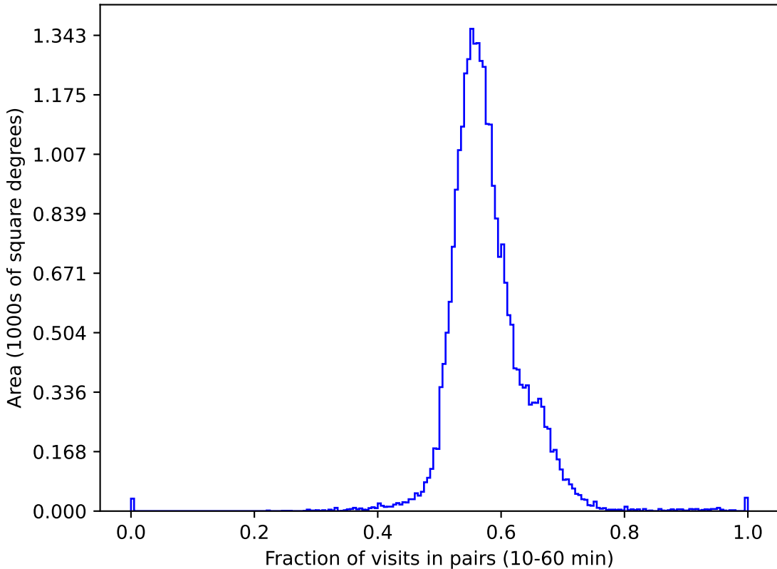
weather_cloudso14v3.4_10yrs gri All sky: Fraction of visits in pairs (10-60 min)
