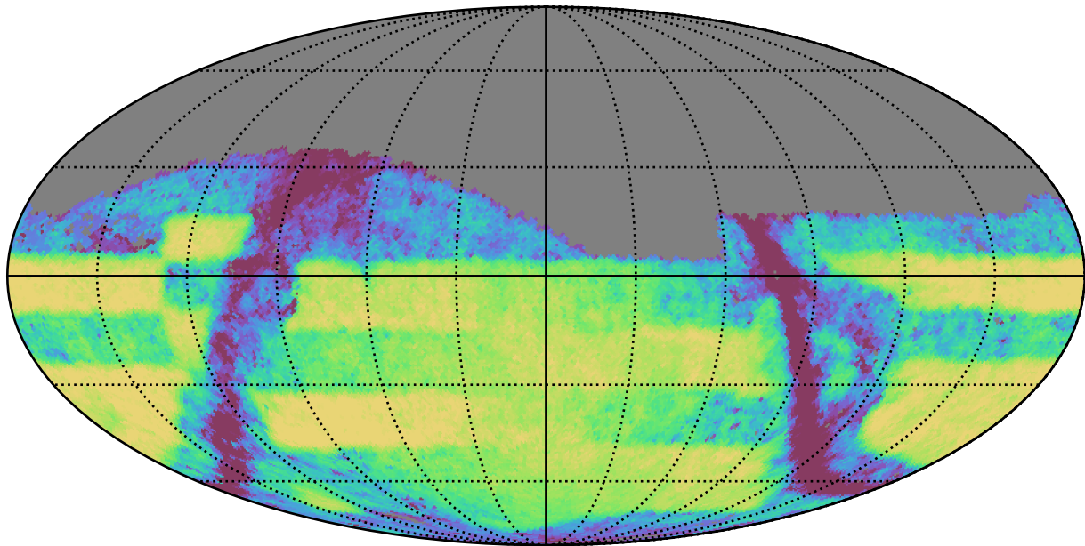
weather_cloudso14v3.4_10yrs Yr 3-4 z band: Exgal_CoaddM5
