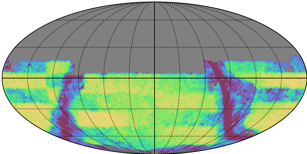
weather_cloudso14v3.4_10yrs Yr 3-4 y band: Exgal_CoaddM5
