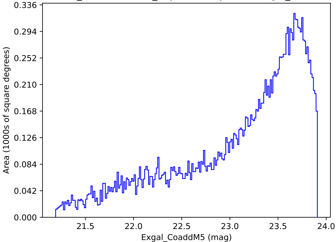
weather_cloudso14v3.4_10yrs Yr 3-4 y band: Exgal_CoaddM5
