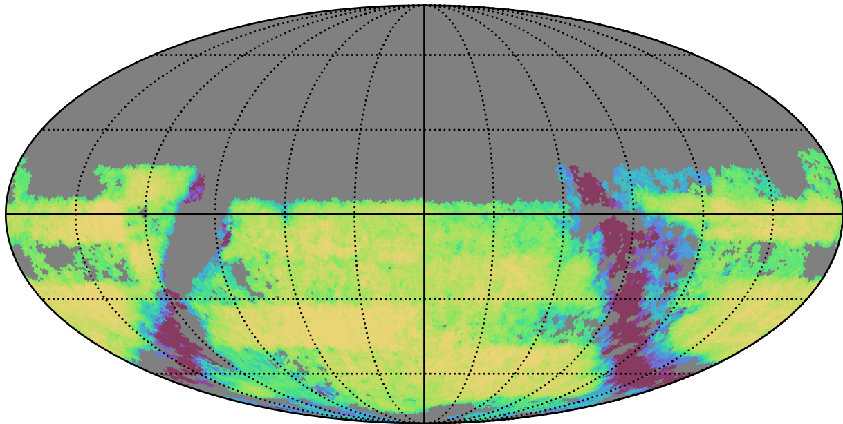
weather_cloudso14v3.4_10yrs Yr 3-4 u band: Exgal_CoaddM5
