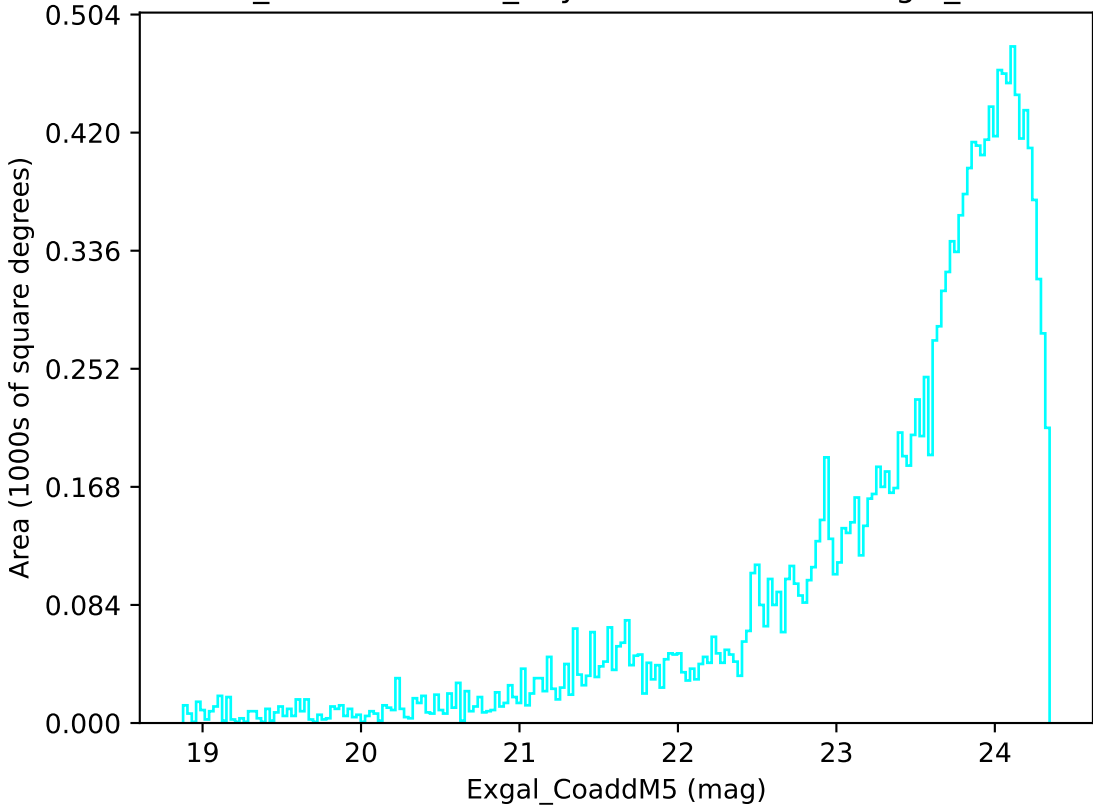
weather_cloudso14v3.4_10yrs Yr 3-4 u band: Exgal_CoaddM5
