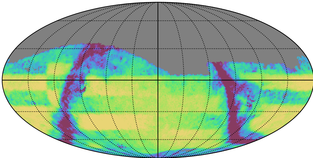
weather_cloudso14v3.4_10yrs Yr 3-4 r band: Exgal_CoaddM5
