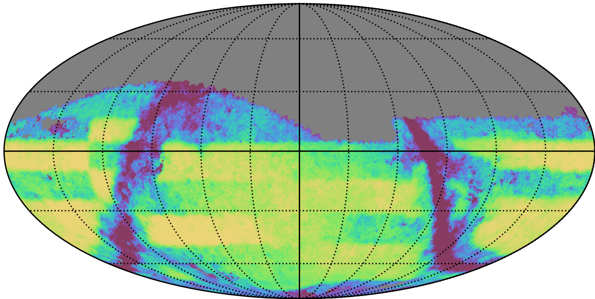
weather_cloudso14v3.4_10yrs Yr 3-4 i band: Exgal_CoaddM5
