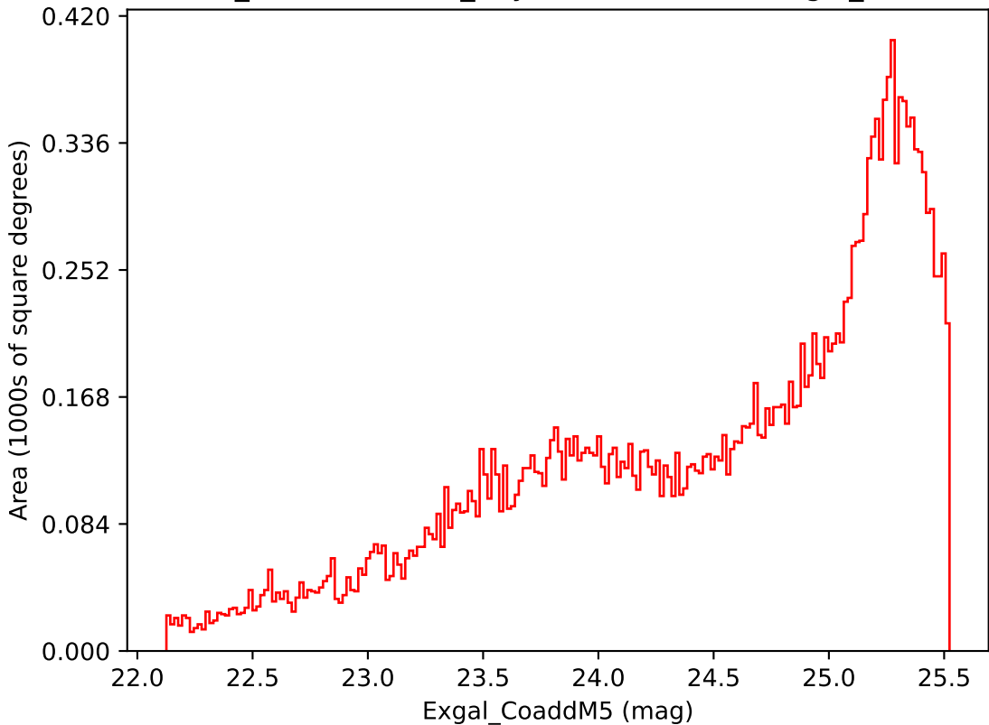
weather_cloudso14v3.4_10yrs Yr 3-4 i band: Exgal_CoaddM5
