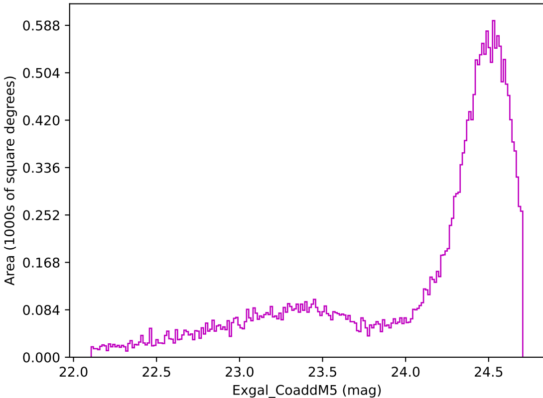
weather_cloudso14v3.4_10yrs Yr 1 z band: Exgal_CoaddM5
