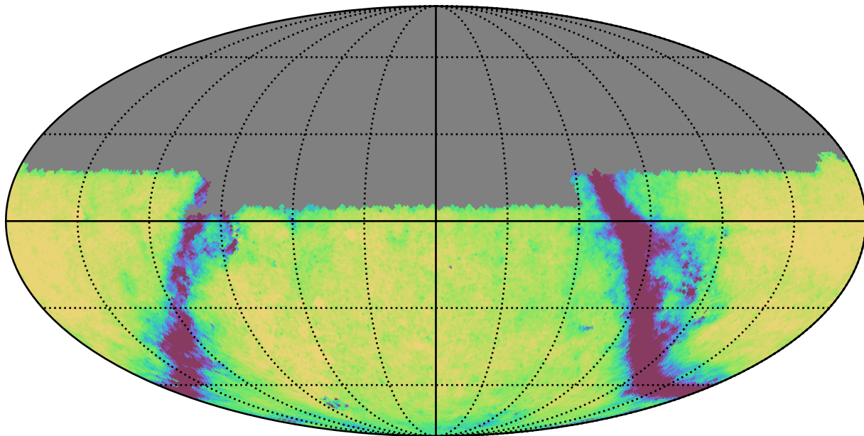
weather_cloudso14v3.4_10yrs Yr 1 u band: Exgal_CoaddM5
