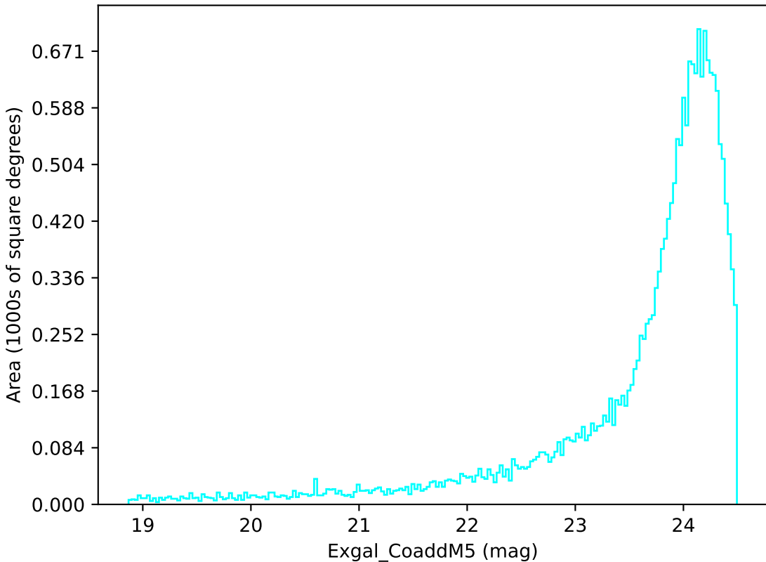
weather_cloudso14v3.4_10yrs Yr 1 u band: Exgal_CoaddM5
