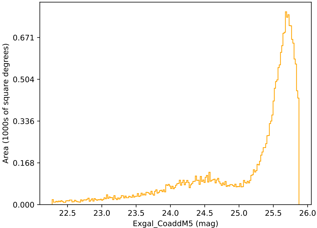
weather_cloudso14v3.4_10yrs Yr 1 r band: Exgal_CoaddM5
