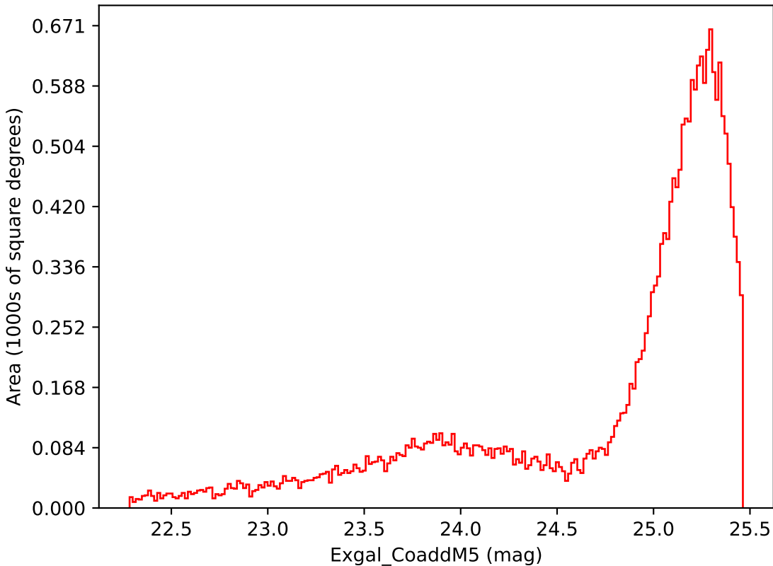
weather_cloudso14v3.4_10yrs Yr 1 i band: Exgal_CoaddM5
