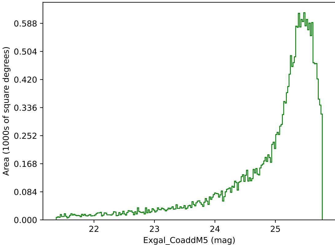
weather_cloudso14v3.4_10yrs Yr 1 g band: Exgal_CoaddM5
