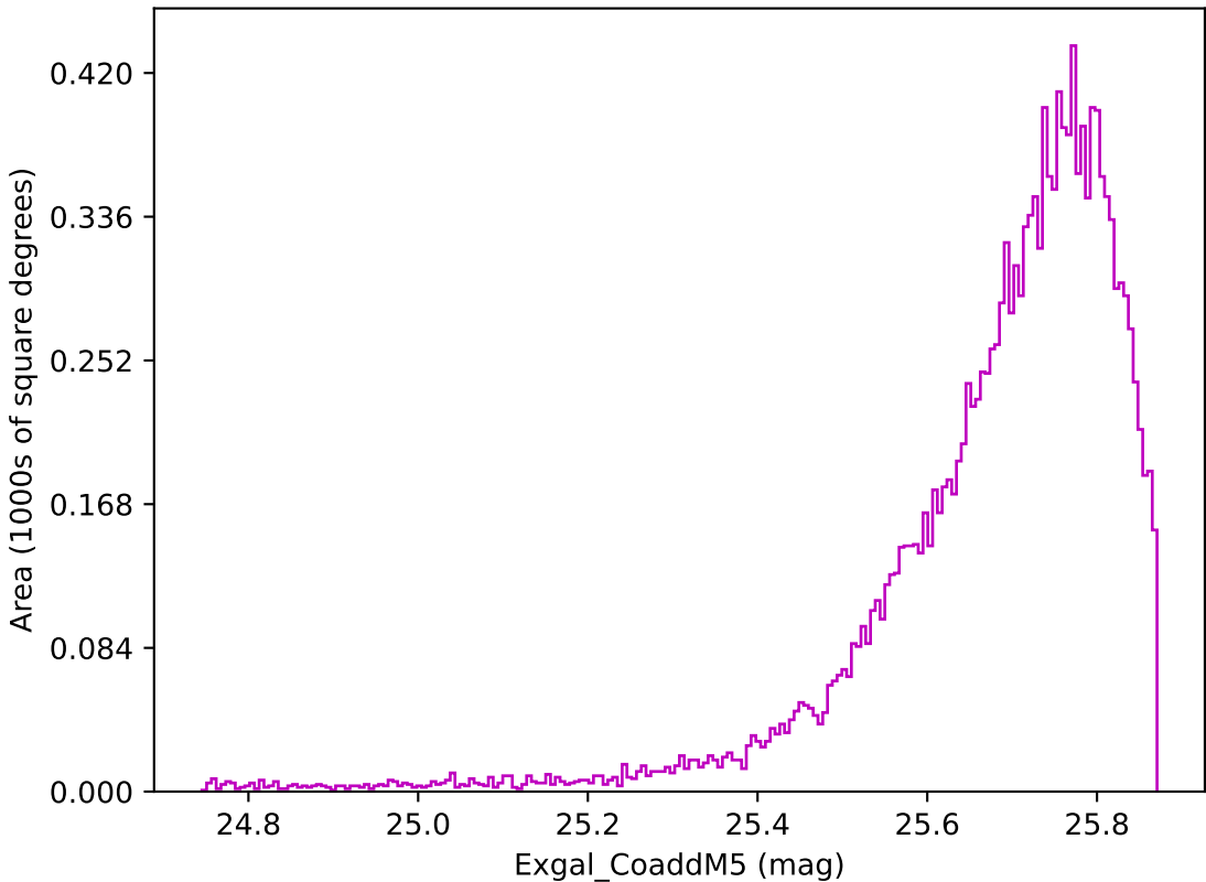
weather_cloudso14v3.4_10yrs WFD z band: Exgal_CoaddM5
