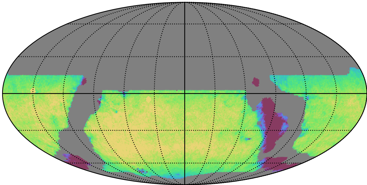
weather_cloudso14v3.4_10yrs WFD y band: Exgal_CoaddM5
