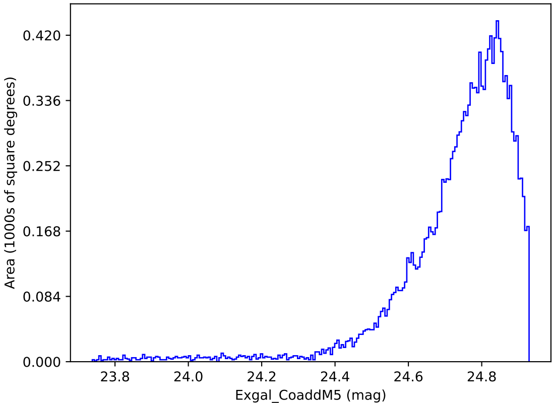
weather_cloudso14v3.4_10yrs WFD y band: Exgal_CoaddM5
