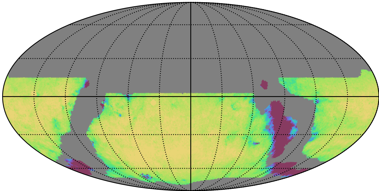
weather_cloudso14v3.4_10yrs WFD u band: Exgal_CoaddM5
