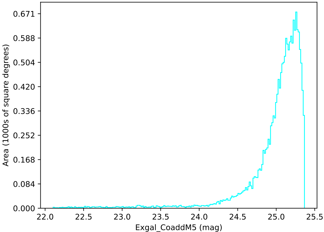
weather_cloudso14v3.4_10yrs WFD u band: Exgal_CoaddM5
