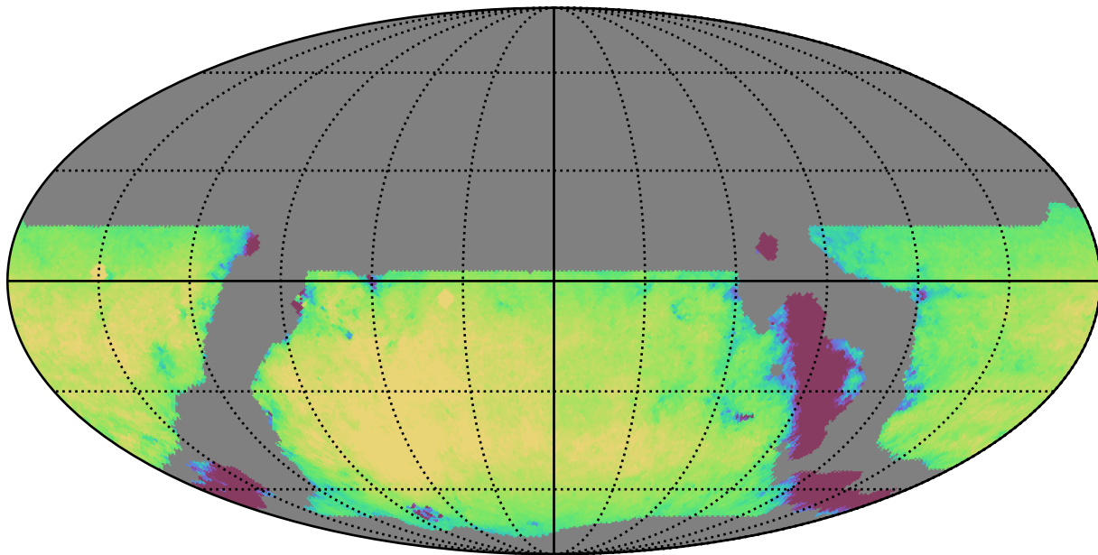
weather_cloudso14v3.4_10yrs WFD r band: Exgal_CoaddM5
