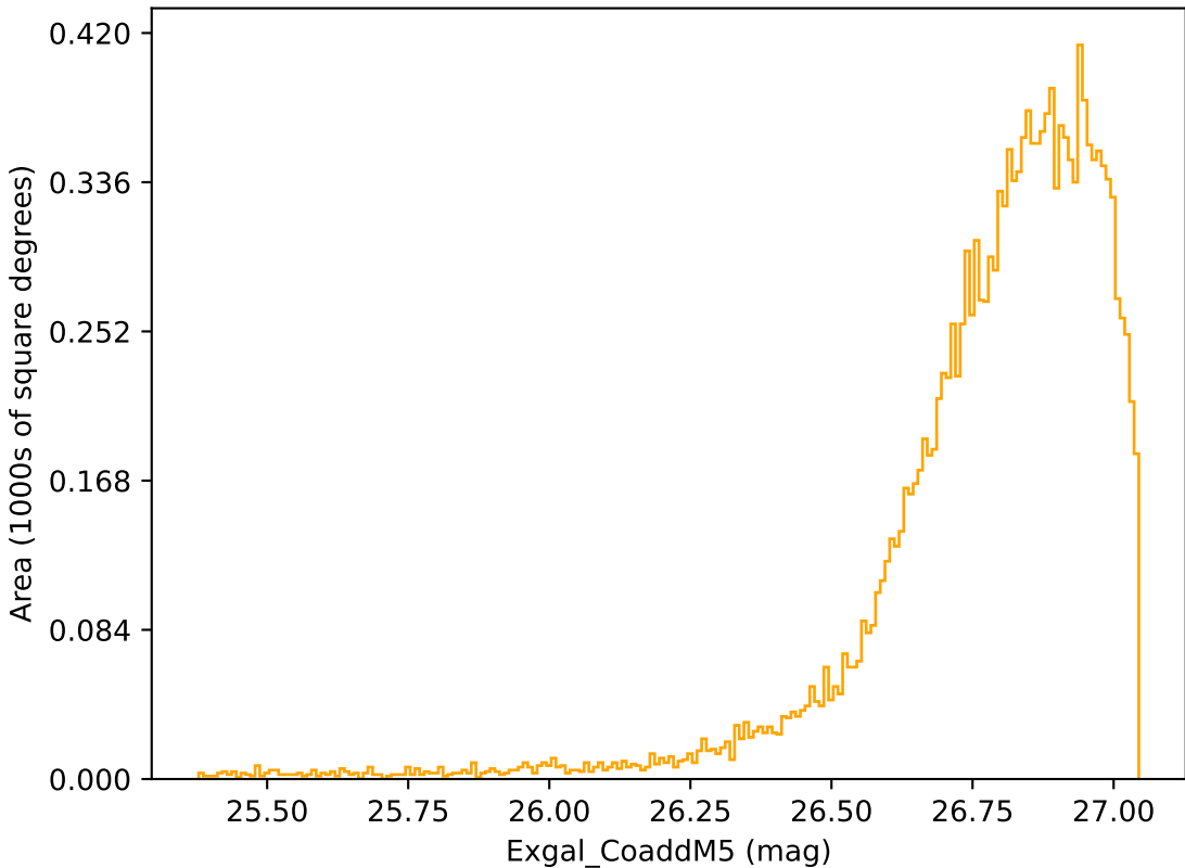
weather_cloudso14v3.4_10yrs WFD r band: Exgal_CoaddM5
