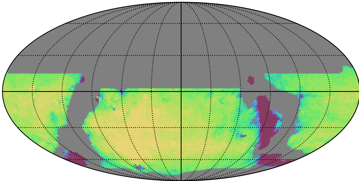
weather_cloudso14v3.4_10yrs WFD g band: Exgal_CoaddM5
