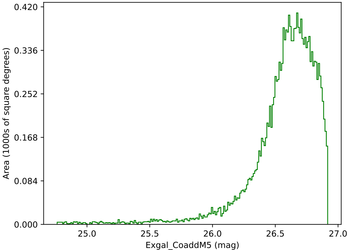
weather_cloudso14v3.4_10yrs WFD g band: Exgal_CoaddM5
