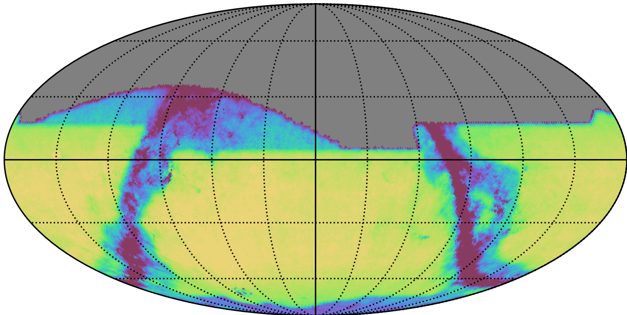
weather_cloudso14v3.4_10yrs All sky z band: Exgal_CoaddM5
