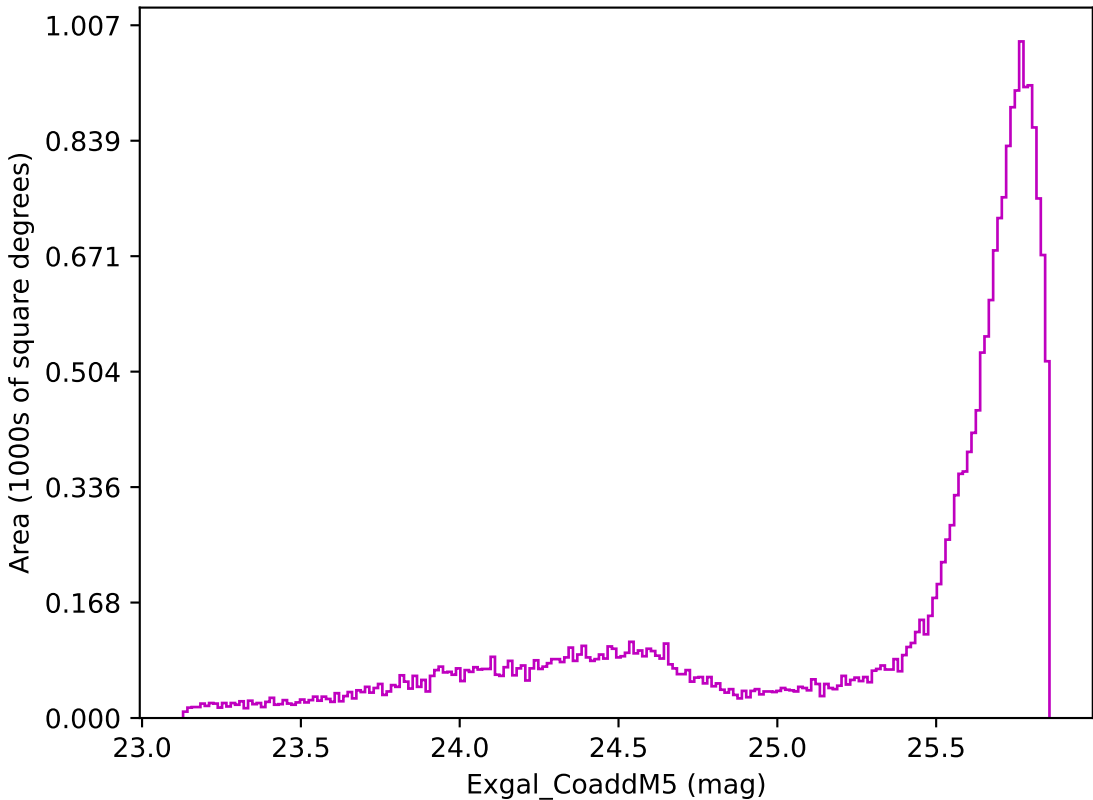
weather_cloudso14v3.4_10yrs All sky z band: Exgal_CoaddM5
