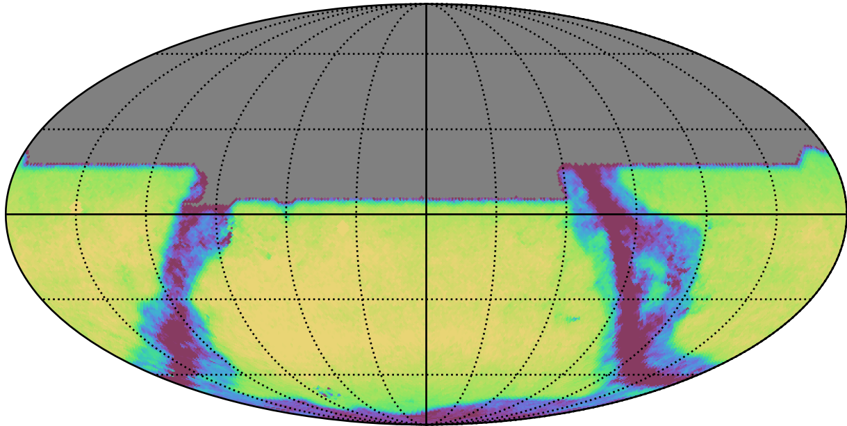
weather_cloudso14v3.4_10yrs All sky y band: Exgal_CoaddM5
