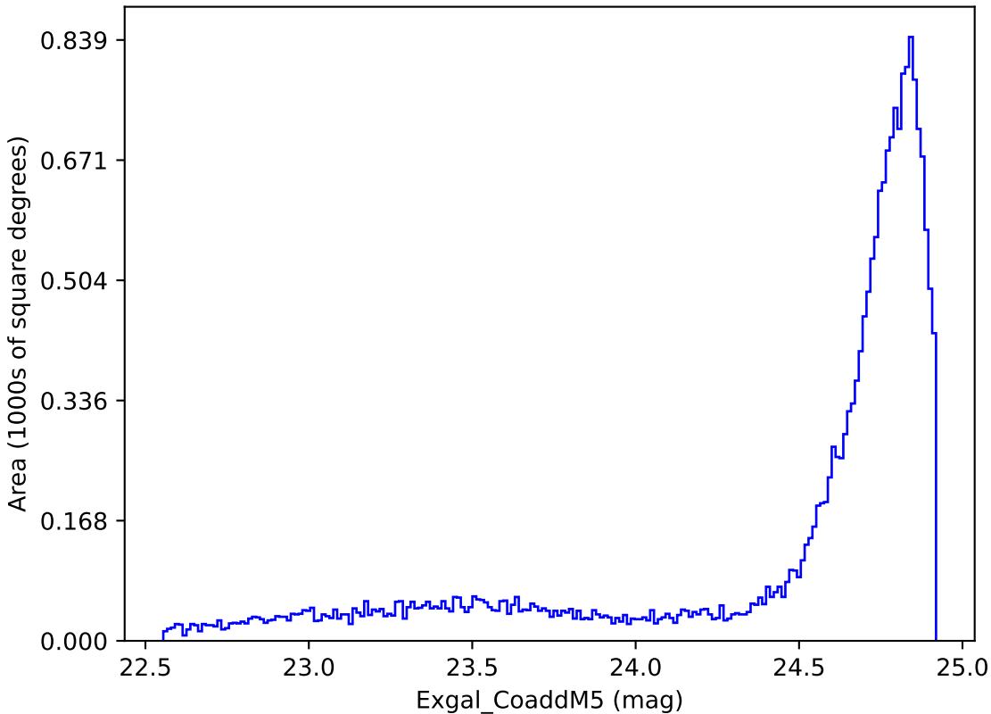
weather_cloudso14v3.4_10yrs All sky y band: Exgal_CoaddM5
